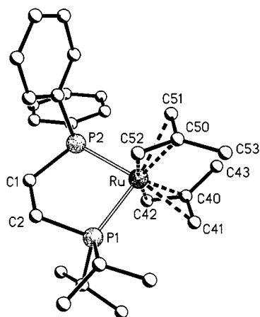
Figure 1. Molecular structure of compound 2 ; selected bond lengths [Å] and angles [°]: Ru–P1 2.3278(9), Ru–P2 2.2981(8), Ru–C40 2.178(3), Ru–C41 2.237(4), Ru–C42 2.232(4), Ru–C50 2.181(3), Ru–C51 2.247(3), Ru–C52 2.230(4), P1–C2 1.854(3), P2–C1 1.851(3); P1–Ru–P2 85.32(3), C1–P2–Ru 110.07(11), C2–P1–Ru 107.03(11), C1–C2–P1 111.9(2), C2–C1–P2 110.1(2), C41–C40–C42 116.4(3), C51–C50–C52 117.9(3).
