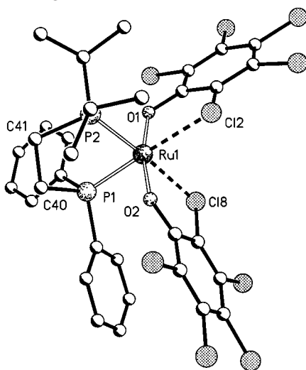
Figure 2. Molecular structure of compound 6 ; the THF molecule is omitted for clarity; selected bond lengths [Å] and angles [°]: Ru–P1 2.2341(13), Ru–P2 2.2578(13), Ru–O1 2.088(3), Ru–O2 2.078(3), Ru–Cl2 2.5240(13), Ru–Cl8 2.4978(13); P1–Ru–P2 84.32(5), P1–Ru–O1 99.45(9), P1–Ru–O2 89.24(9), P1–Ru–Cl2 176.70(4), P1–Ru–Cl8 94.03(5), P2–Ru–O1 94.51(9), P2–Ru–O2 93.00(8), P2–Ru–Cl2 98.90(5), P2–Ru–Cl8 174.32(4), O1–Ru–O2 169.03(11), O1–Ru–Cl2 79.60(9), O1–Ru–Cl8 91.12(9), O2–Ru–Cl2 91.34(9), O2–Ru–Cl8 81.53(8), Cl2–Ru–Cl8 82.85(4).
